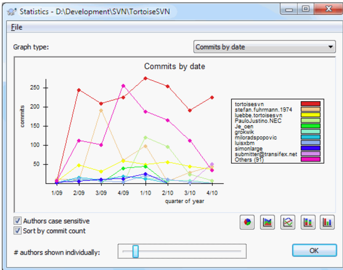
Figure 4.25. Commits-by-date Graph
