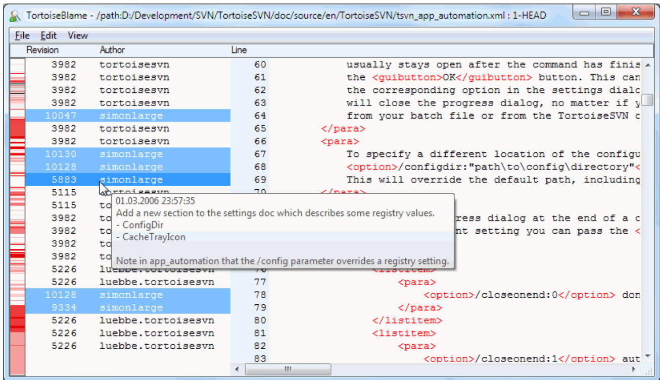
Figure 4.61. TortoiseBlame
