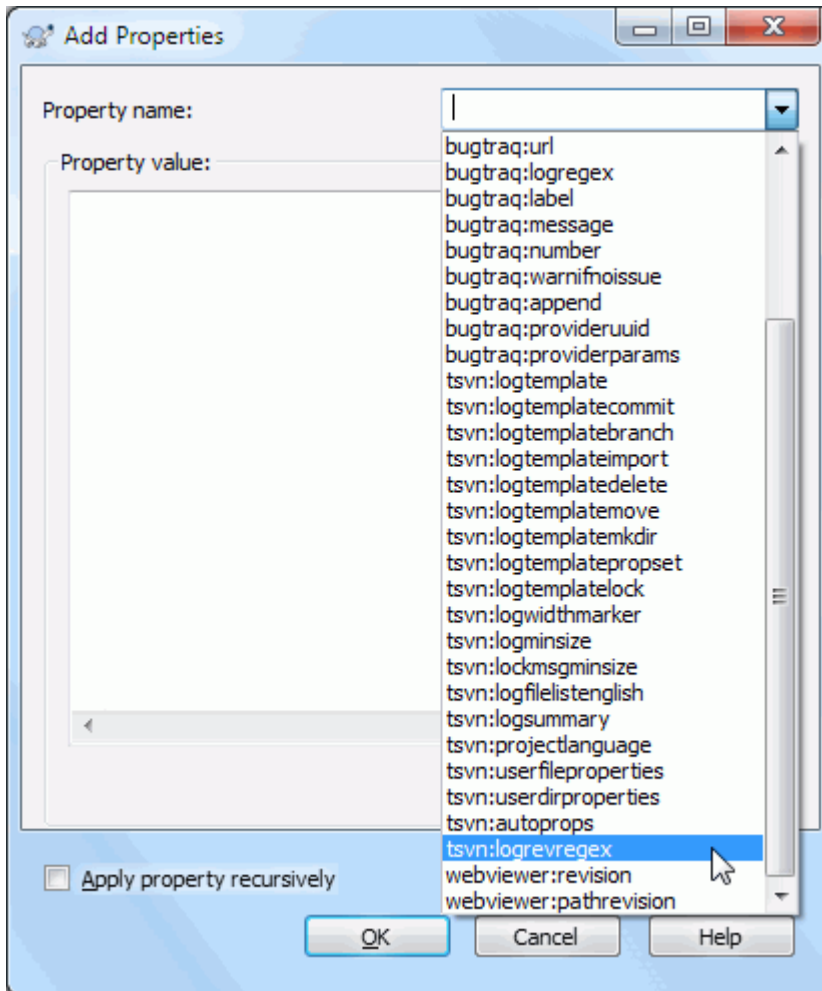
Figure 4.35. Adding properties
