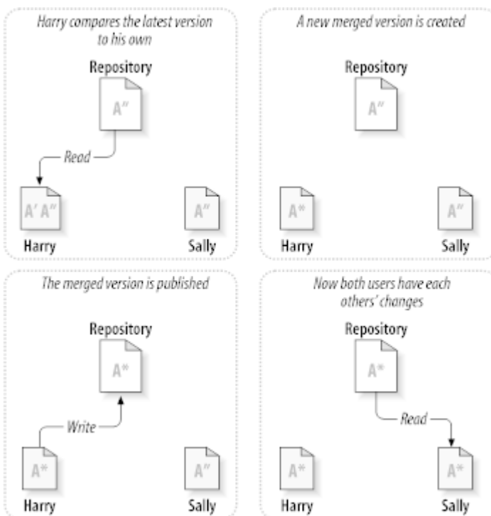
Figure 2.5. ...Copy-Modify-Merge Continued
