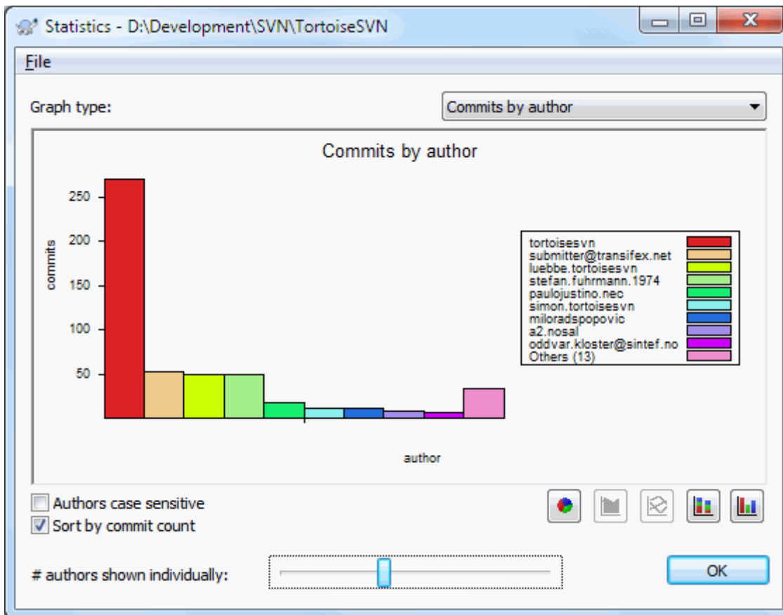
Figure 4.23. Commits-by-Author Histogram
