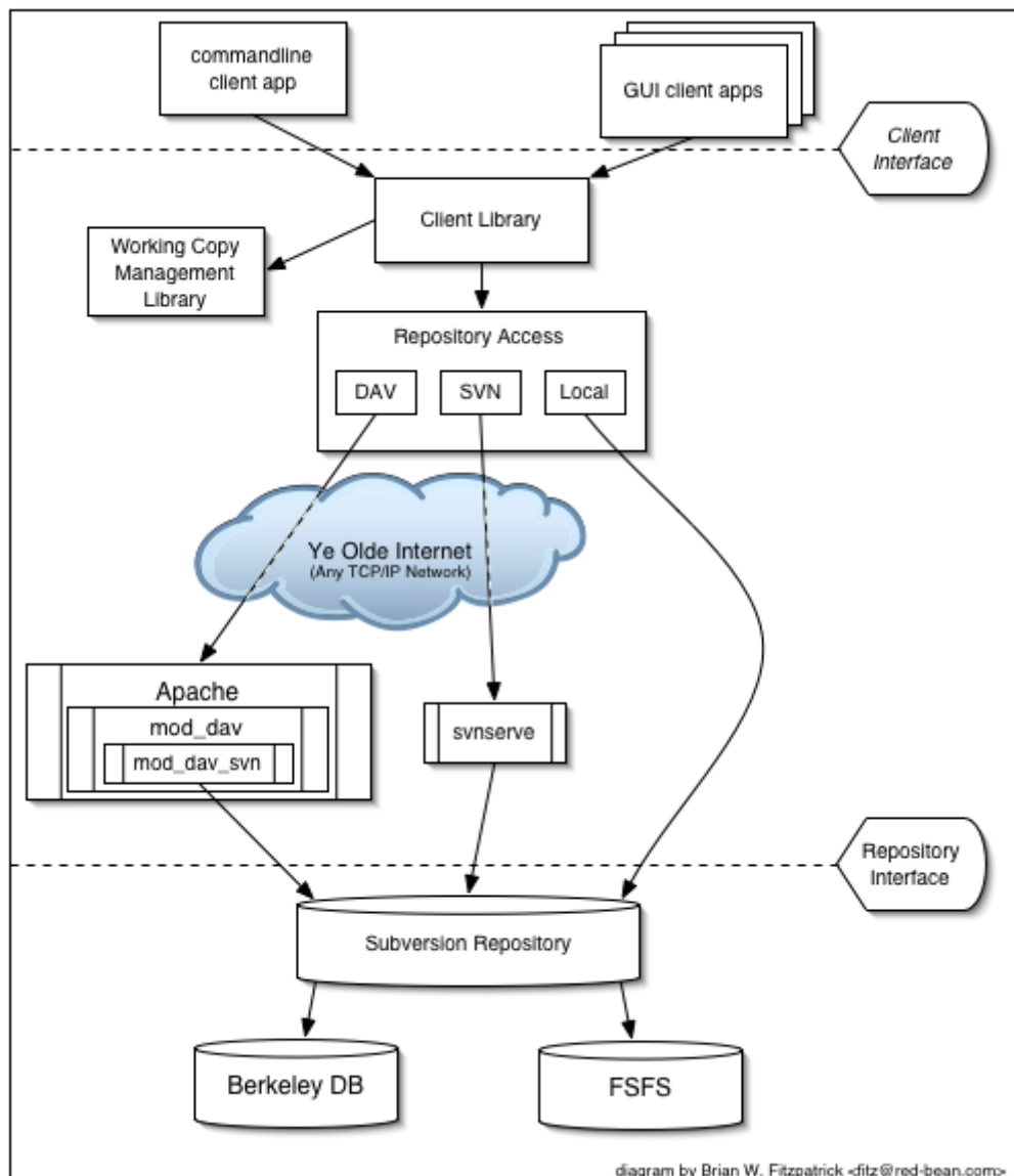
Figure 1. Subversion's architecture
